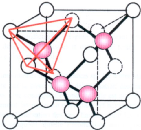
Diamant cubique
