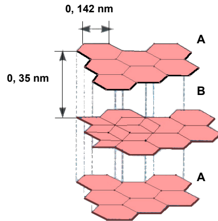
Graphite hexagonal
