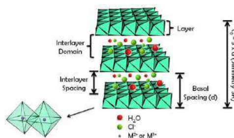
Figure 1. Schematic representation of LDH structure.
