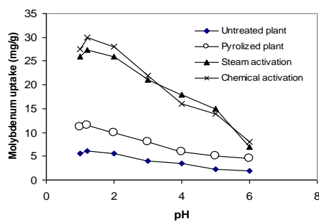
Figure 2 : pH effect on Mo uptake.
