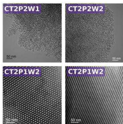
Figure 1. Mesoporous carbons synthesised using different P:W weight ratios.
