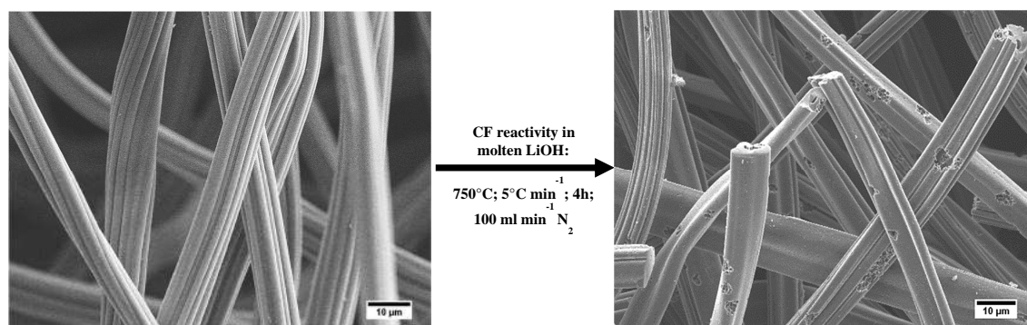
Figure 1 : SEM micrographs of CF fibers; a)-before and b)-after prolonged contact with molten LiOH in the conditions given below the arrow.
